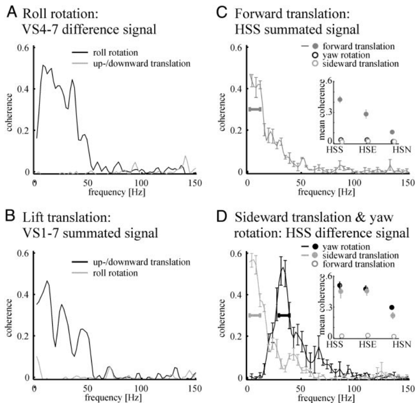
FIG. 5. Population coding of self-motion: coherences between cardinal self-motion components and the population response that leads to the highest coherence. A : coherence between intersaccadic roll rotation and a composite response obtained by subtracting the summated response of ipsilateral VS4-7 neurons from the summated 4 responses of the corresponding contralateral neurons (4 neuron pairs). Coherence between intersaccadic upward/downward velocity and the composite response is negligible. B : coherence between intersaccadic upward/downward velocity and the sum over 7 representative ipsilateral responses and the 7 corresponding contralateral responses from VS1-7 neurons (7 neuron pairs). Coherence between intersaccadic roll velocity and the summated response of ipsi- and contralateral VS1-7 neurons is negligible. C : coherence between the summated responses of the left and right HSS neuron and the intersaccadic forward velocity (average and SE of 3 HSS neurons). Inset : mean coherences of the summated response of the left and right neurons for all HS neurons (HSN, 9 neurons; HSE, 7 neurons; HSS, 3 neurons). Coherence was averaged over a 10-Hz window, centered near the maximum coherence. Coherences between the summated responses of the left and right HS neurons and yaw and sideward velocity is negligible for all 3 HS types. D : difference signal between the left and right HSS neurons produces high coherences with both intersaccadic yaw and sideward velocity (average of 3 HSS neurons). Inset : mean coherences of the difference signal for all HS neurons (HSN, 9 neurons; HSE, 7 neurons; HSS, 3 neurons). Coherences were averaged over 10-Hz windows. Coherence between the difference response of all 3 HS neuron types and forward velocity is negligible. All coherences were calculated for the intersaccadic intervals.
