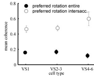
FIG. 4. Mean coherences between tangential neurons' responses and the "no translation" stimulus (NT). A : mean coherence of a neuron from the VS4-6 group neurons calculated for the rotation around the preferred axis for the entire NT flight and between the saccades (mean and SE). Horizontal bars in A and B denote the frequency range used to calculate the mean coherences shown in C and D . B : coherence between the HSN neurons' responses and yaw rotation for the entire flight and between the saccades. C : mean coherences for 3 groups of VS neurons calculated for the preferred rotation axis for the entire stimulus and between the saccades. D : mean coherences for the 3 HS neuron types calculated for yaw rotation for the entire NT stimulus and between the saccades. Mean coherences are averages over the right and left neuron (VS1, 5 neurons; VS2-3, 3 neurons; VS4-6, 4 neurons; HSN, 8 neurons; HSE, 2 neurons; HSS, 1 neuron). Error bars show SE.
