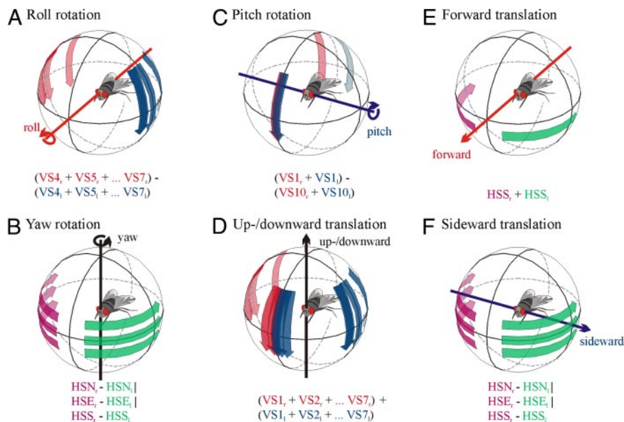
FIG. 6. Population coding of self-motion: neuronal populations appropriate for the encoding of self-motion around and along all 3 cardinal axes. A–C: specificity to self-rotation is enhanced by subtracting the responses of 2 sets of neurons from opposite sides of the visual sphere having the same preferred rotation axis but opposite preferred rotation directions. A: subtracting responses of a group of heterolateral VS neurons with laterally located receptive fields increases the specificity to roll rotation. B: subtracting responses of heterolateral HS neuron pairs (HSN, HSE, and HSS) increases the specificity to yaw rotation. C: subtracting responses of VS neurons with frontally and caudally located receptive fields should increase the specificity to pitch rotation. D–F: specificity to self-translation is enhanced by summing responses of neurons exhibiting the same sensitivity or by subtracting neurons with opposite sensitivity to the respective self-motion. D: summing responses of all recorded VS neuron types enhances the specificity to up-/downward translation. E: summing responses of heterolateral HSS neurons with ventrally located receptive fields increases the specificity to forward translation. F: subtracting responses of heterolateral HS neuron pairs (HSN, HSE, and HSS) increases the specificity to sideward translation.
