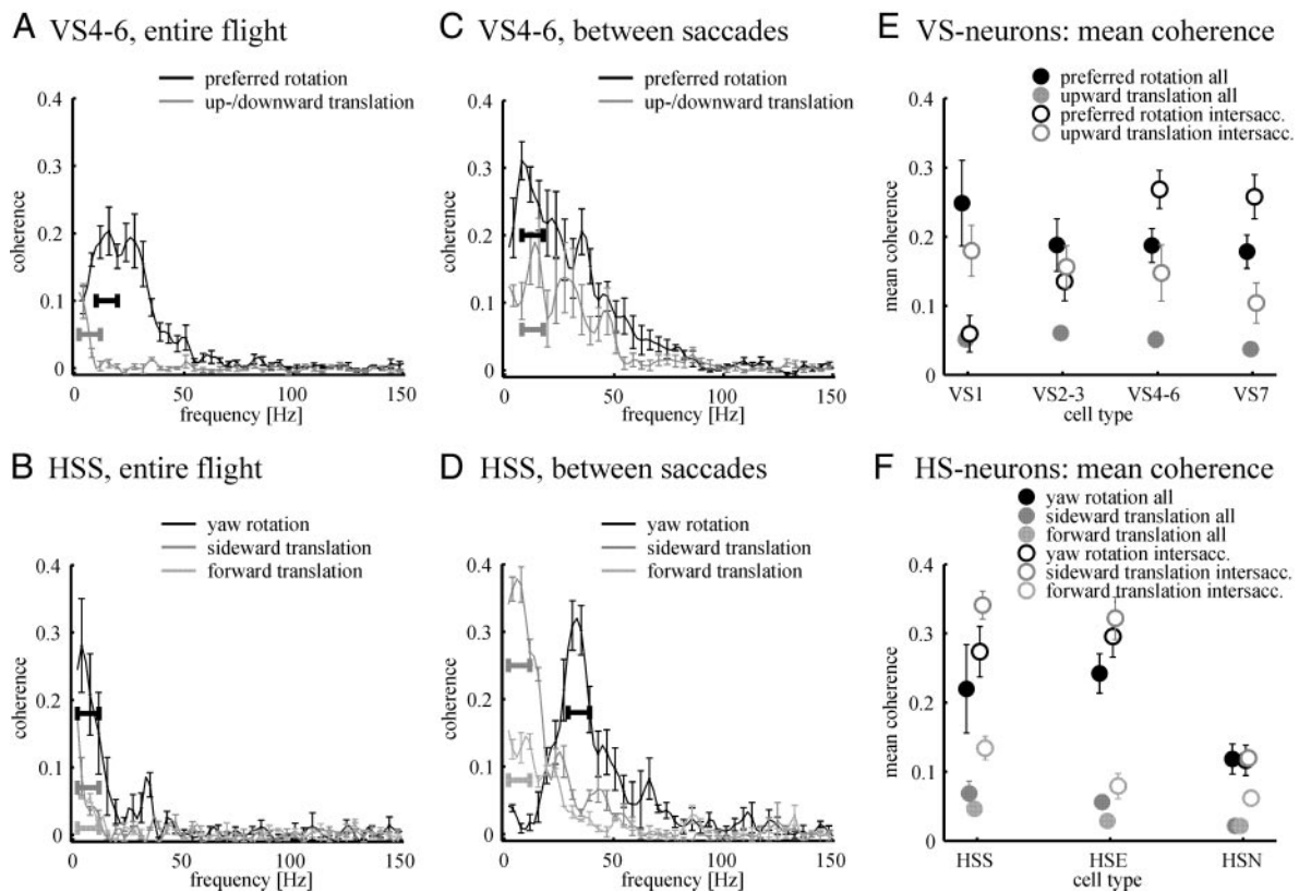
FIG. 3. Coherences between responses of tangential neurons and rotational or translational velocities. A : mean and SE of the coherence between the response (entire flight) of each VS4-6 neuron and the rotational velocity around its preferred rotation axis, and coherence with upward/downward velocity. Preferred rotation axis was obtained from the tuning curve calculated from coherence rates (cf. Fig. 2 B ). Horizontal bars in A–D denote the integration windows used to calculate the mean coherences shown in E and F . For clarity, error bars are shown for only every other data point. B : coherence between the HSS neuron response and a preferred axis rotation, sideward and forward translation for the entire flight. We assumed the yaw axis as the preferred rotation axis of HS neurons. C : as in A , for the response in the periods between the saccades. D : coherence between the HSS neuron response and a preferred rotation, sideward and forward translation for the periods between the saccades. Coherences in C and D were calculated by masking out the saccadic part of the stimulus and the neuronal response (cf. METHODS). E : mean coherences of all VS neuron types for a preferred axis rotation and an upward/downward translation for the entire flight and between the saccades. Frequencies were averaged over a frequency band of 10 Hz, centered near the maximum coherence for each condition. F : mean coherences of all HS neuron types for preferred rotation (yaw), sideward translation, and forward translation for the entire flight and between the saccades. All coherences and mean coherences are averages over the right and left neurons (VS1, 5 neurons; VS2-3, 4 neurons; VS4-6, 8 neurons; VS7, 1 neuron; HSN, 9 neurons; HSE, 8 neurons; HSS, 9 neurons). Error bars show SE.
