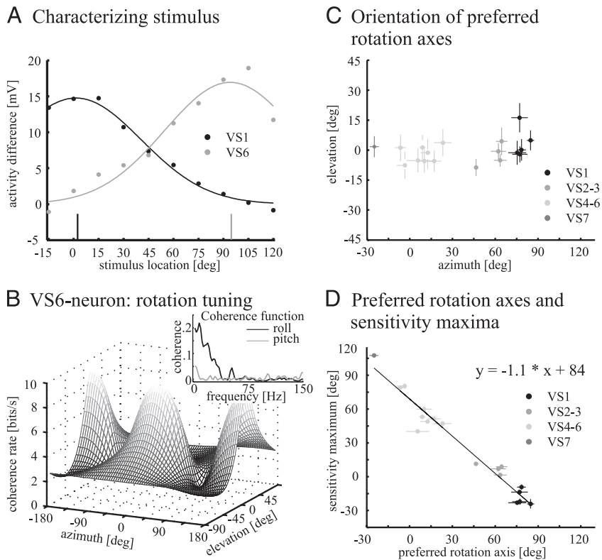
FIG. 2. Classification of VS neurons and determination of the respective preferred rotation axis. A : receptive field as determined by the difference between the neuronal responses to an up- and downward moving dot for a VS1 and a VS6 neuron. Difference responses are plotted as a function of the stimulus positions along the azimuth. Gaussian functions are fitted to the measured data of the 2 neurons. Arrows pointing at the x -axis denote the maximum of the fits and can be regarded as the sensitivity maximum of the respective neurons. B : tuning curve of the VS6 neuron to rotation obtained from the coherence rate. Inset : coherence functions between the VS6 neuron's response and the roll and pitch velocity. Coherence rate was calculated from the coherence function over a frequency range from 1 to 150 Hz. To obtain the tuning curve, the coherence rate was calculated for head rotations around axes in a 2-D grid. Azimuth between -180 (roll-axis) and 175^\circ , elevation between -90 and 85^\circ ( 5^\circ steps). Azimuth value of -90/90^\circ corresponds to the pitch axis. C : azimuth and elevation of the average preferred rotation axes for all VS neurons recorded in the experiments. An average axis and corresponding SE were calculated by weighting the axis for each stimulus condition, obtained from the peak of a tuning curve as presented in B , with the coherence rate at the respective peak. D : preferred rotation axes as a function of receptive fields' sensitivity maxima calculated as shown in A (mean and SE). Linear regression line fitted to the data has a slope of -1.1 .
