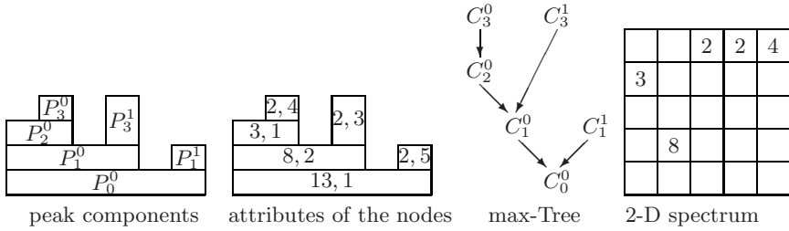
Fig. 1. Peak components( P_h^k ), their attributes, corresponding ( C_h^k ) (the max-tree) and the resulting pattern spectrum (right)
