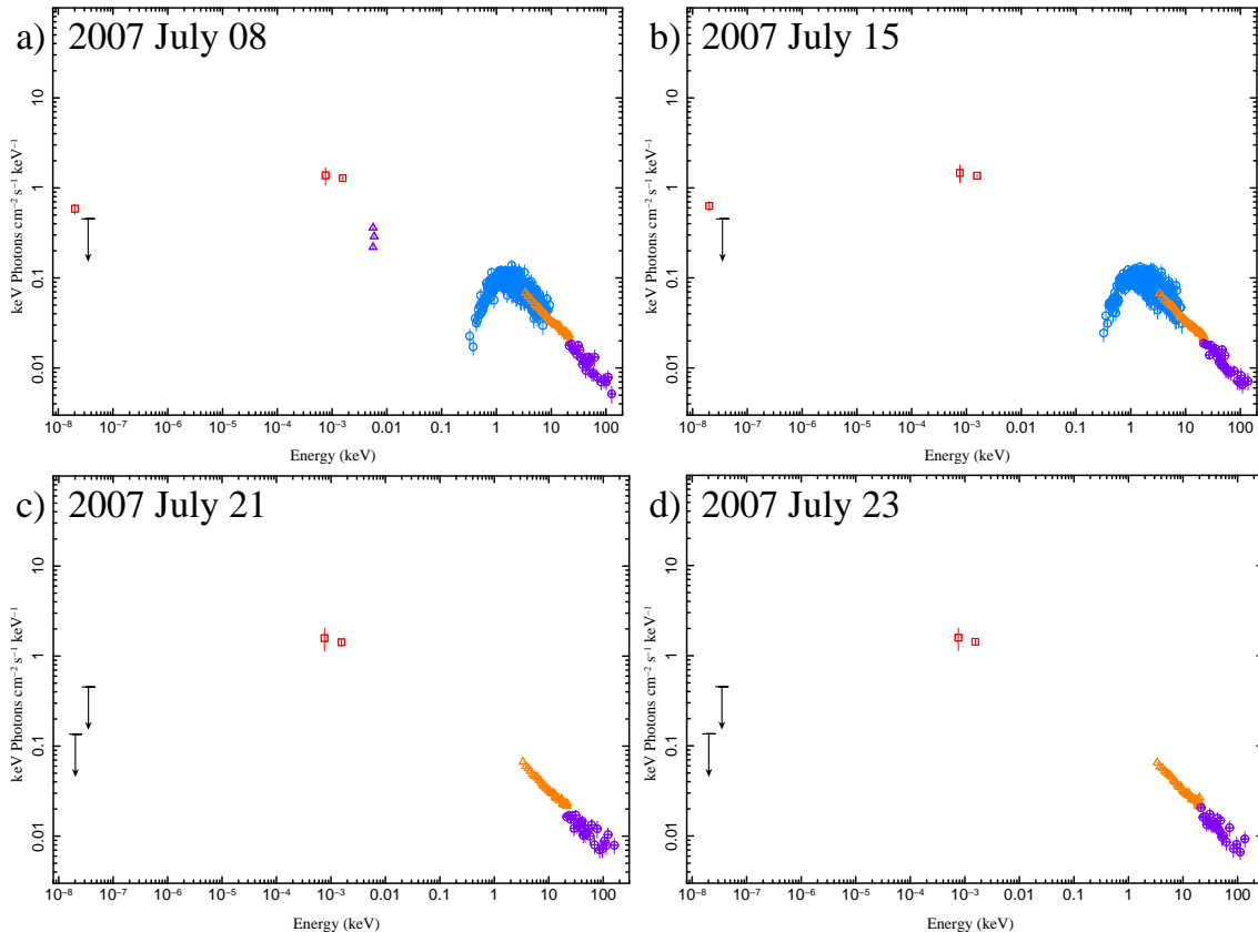
Figure 7. SEDs of Swift J1753.5-0127 on 2007 July 08, 15, 21 and 23 (panels a, b, c and d, respectively). We are showing the observed OIR, ultraviolet and X-ray fluxes, without correcting for the absorption. The red squares and the black arrows on the left-hand side of each panels mark the radio WSRT observations (detections at 4.9 GHz and 3\sigma upper limit at 8.5 GHz). The red squares (at an energy of \sim 10^{-3} keV) represents the H and I bands detections with SMARTS. The Swift/UVOT detections (ultraviolet, available only for panel a) are marked with purple triangles. X-ray points are marked with blue open circles (Swift/XRT, not available for panels c and d), orange open triangles (RXTE/PCA) and purple open circles (RXTE/HEXTE). See §2 for the details on the data reduction and Tables 1, 2 and 3 for the values of the used fluxes. Panel c): we used WSRT and RXTE data from 2007 July 22 and SMARTS data from 2007 July 21. Panel d): we used WSRT and RXTE data from 2007 July 22 and SMARTS data from 2007 July 23.
