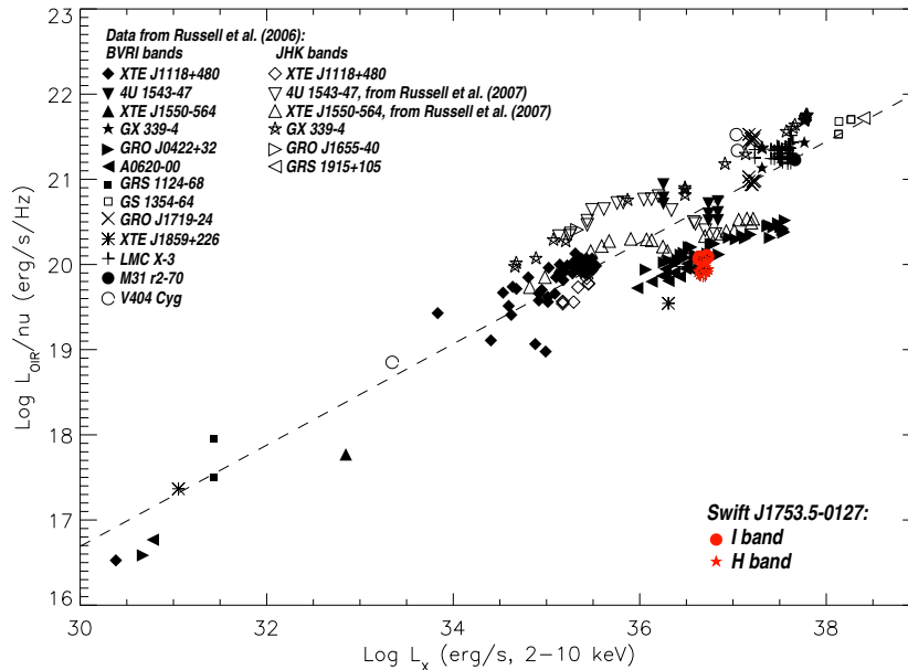
Figure 6. The BHCs sample of Russell et al. (2006), with the addition of the Swift J1753.5-0127 data. We also included data from the BHCs XTE J1550-564 and 4U 1543-47 (near IR only), from Russell et al. (2007). The dashed line is the fit to the Russell et al. (2006) data, a relation of the form L_{OIR} \propto L_X^{0.61 \pm 0.02} in the (L_X, L_{OIR}) plane. Our data of Swift J1753.5-0127 are marked in red, for the two bands (I and H). We did not plot the error bars for clarity.
