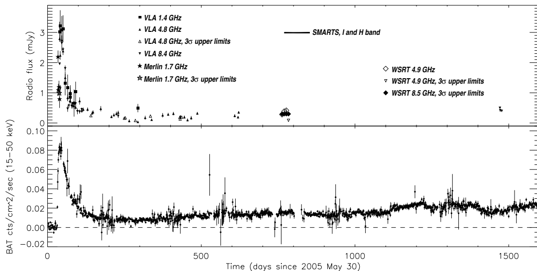
Figure 1. Lower panel: Swift/BAT light curve of Swift J1753.5-0127 for the period 2005 May 30 - 2009 October 16. Bin size is 1 day. The dashed line marks the zero of the y axis. Upper panel: radio light curve of Swift J1753.5-0127. We plotted all our data points (VLA, MERLIN and WSRT). Bin size is a whole observation. The horizontal thick line marks the period in which we performed SMARTS OIR observations (H and I band). A complete log of all the radio and OIR observations is reported in the appendix (§A).
