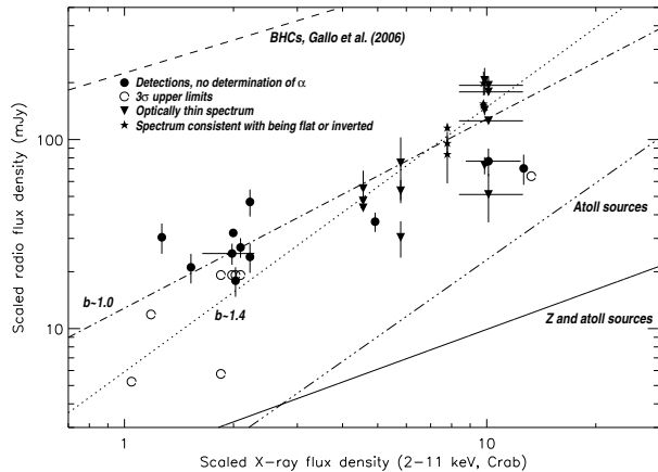
Figure 8. Zoom of Figure 3, in which only the data points from Swift J1753.5-0127 are reported. A key to the different symbols is also shown. We determined the radio spectral index only for those observations with detections at three (or more) frequencies. The dashed, dotted-dashed and dotted lines have already been defined in §3.1 and in the caption of Figure 3. The solid line and the dashed-dotted-dotted line represent the best fits reported in Figure 2 of Migliari & Fender (2006) for the atoll and Z sources ( k \sim 1.98 , b \sim 0.7 ) and the atoll sources only ( k \sim 1.03 , b \sim 1.35 ), respectively.
