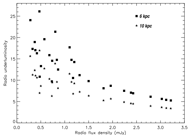
Figure 5. Radio underluminosity of Swift J1753.5-0127 as a function of the radio flux density density for two other possible distances to the source. Different symbols mark the two distances (6 and 10 kpc). On the X axis we plotted the radio flux density and not the scaled radio flux density, as we did in Figure 3 and Figure 4. We considered only the radio detections and not the 3\sigma upper limits.
