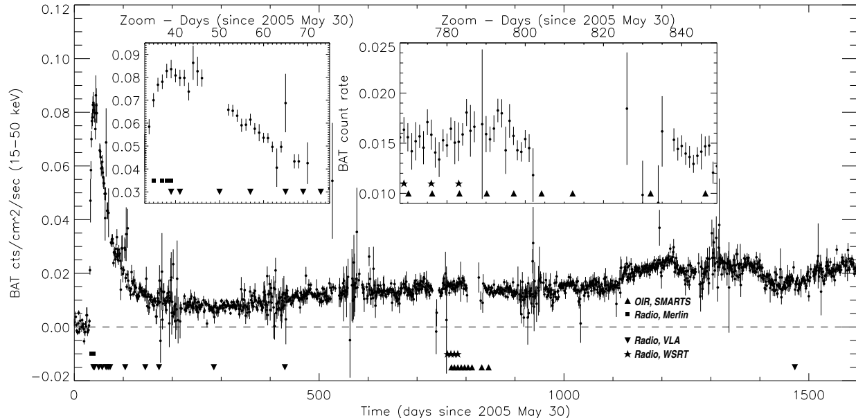
Figure 2. Swift/BAT light curve of Swift J1753.5-0127, as in Figure 1. Different symbols at the lower edge of the figure represent the radio (VLA, MERLIN and WSRT) and SMARTS observations listed in Tables 2 and 3. For clarity, the insets show a zoom on two intervals (2005 July 02 - 2005 August 13 and 2007 July 07 - 2007 August 26).
