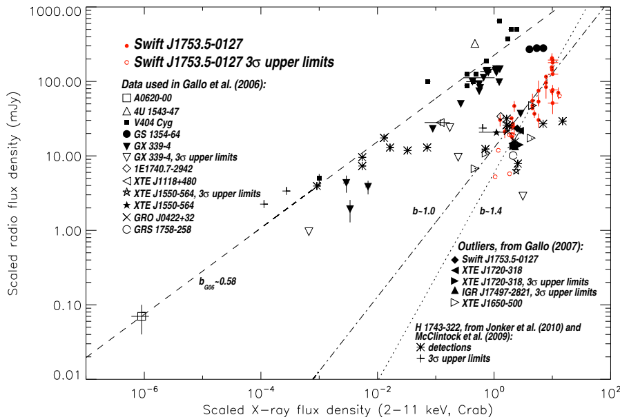
Figure 3. The BHCs sample of Gallo et al. (2006) and Gallo (2007), with the addition of the Swift J1753.5-0127 data (red points). We also included data from the BHC H 1743-322, recently reported in McClintock et al. (2009) and Jonker et al. (2010). The X-ray scaled fluxes from McClintock et al. (2009) and Jonker et al. (2010) have been measured in the energy bands 2-20 keV and 0.5-10 keV, respectively. The dashed line is the fit to the Gallo et al. (2006) data, a non-linear relation of the form S_{radio} = k(S_X)^b ( k_{G06} = 224.72 and b_{G06} = 0.58 \pm 0.16 ) where S_{radio} is the scaled radio flux density and S_X is the scaled X-ray flux. The dashed-dotted line and the dotted line represent the best-fit limits to the Swift J1753.5-0127 data, two non linear relations with b \sim 1.0 , k \sim 13 and b \sim 1.4 , k \sim 6 , respectively. Following Gallo et al. (2003) and Gallo et al. (2006), all the fluxes have been scaled to a distance of 1 kpc.
