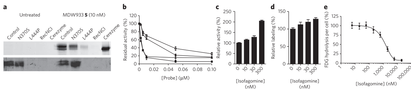
Figure 5 | Labeling of mutant forms of glucocerebrosidase. (a) Detection of GBA in Gaucher fibroblasts by labeling of wild-type and homozygous N370S, L444P and RecNCl collodion fibroblast with 10 nM MDW933 for 60 min. GBA was visualized by in-gel fluorescent scanning (top panel) and by western blotting with 8E4 antibody. For uncut gels, see Supplementary Figure 14 . (b) Inactivation curves of MDW933 (open symbol) and MDW941 (solid symbols) in N370S (triangles) and control fibroblasts (squares). Residual activity was determined with 4-methylumbelliferyl \beta -D-glucopyranoside. Data represent mean values \pm s.d. (c,d) Impact of isofagomine on N370S GBA. In a typical experiment, fibroblasts from the N370S GBA homozygote were incubated with various isofagomine concentrations for 1 week. Data represent mean values \pm s.d. (c) Relative GBA activity in cell lysates observed with 4-methylumbelliferyl \beta -D-glucopyranoside assay after incubating. (d) Quantification of the fluorescent readout of in situ MDW941-labeled GBA activity. (e) Relative lysosomal GBA activity observed as hydrolysis of FDG per cell. Fibroblasts were first treated for 20 min with noted concentrations of isofagomine and subsequently incubated with FDG substrate. FDG fluorescence was assessed by FACS analysis. Data represent mean values \pm s.d.
