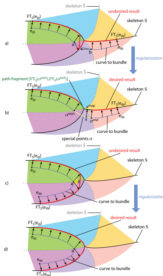
Fig. 3. Attraction singularities. Naive solution (a,c) and corresponding solutions with regularization (b,d). Final bundled curve is shown in red. Voronoi regions of the branches of \bar{S} are shown in different hues.
