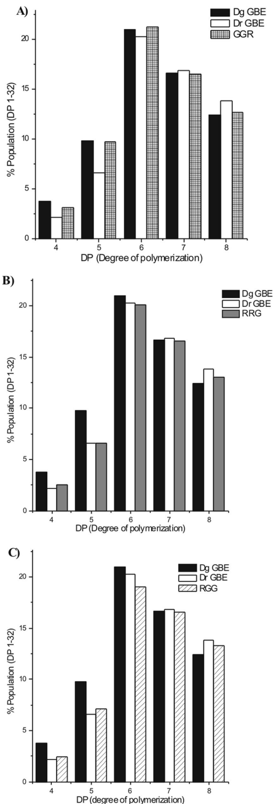
FIG. 5. HPAEC-pulsed amperometric detection analysis of the end products (DP4 to DP8) obtained by incubation of the GBE_{Dg} , GBE_{Dr} or GGR (A), RRG (B), or RGG (C) enzymes with amylose, followed by debranching with isoamylase.
