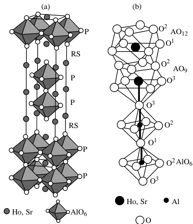
Fig. 1. (a) Unit cell and (b) AlO 6 , AO 9 , and AO 12 coordination polyhedra in Ho 2 SrAl 2 O 7 .
