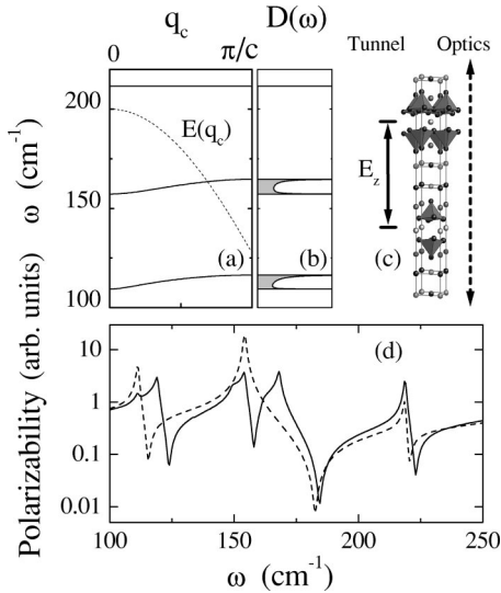
FIG. 6. (a) Simulated phonon dispersion of three branches in the low-frequency range for Bi2212 and q_c dispersion of the electric field in tunneling measurements. (b) The phonon density of states corresponding to the dispersion curves in (a). (c) Tunnel vs optics electric field distribution within the crystal. In the tunneling measurements, the electric field is localized within one junction. (d) Polarizability for the uniform (dashed line) and nonuniform (solid) electric field distribution, simulated on the stack of the ab planes, with each plane representing an atom in the unit cell.
