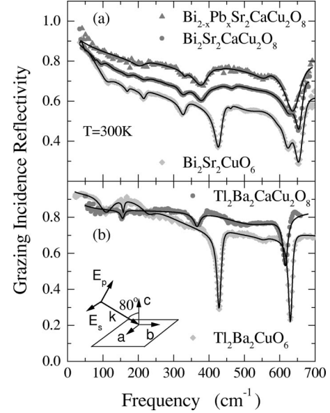
FIG. 1. Experimental (symbols) and fitted (solid lines) grazing angle reflectivity R_p for the p -polarized light measured at an 80^\circ angle of incidence at room temperature for (a) bismuth and (b) thallium compounds. Sketched in the inset is the schematic diagram of the grazing angle technique.
