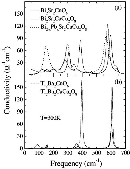
FIG. 2. The c -axis conductivity (a) for the Bi and (b) for Tl compounds, obtained from the fit of the reflectivity to the Drude-Lorentz model.
