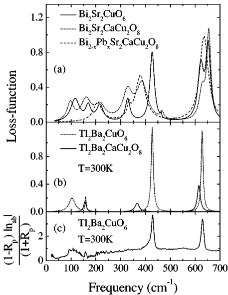
FIG. 3. The c -axis loss function (a) for the Bi and (b) for Tl compounds, obtained from the fit of the reflectivity to the Drude-Lorentz model. Shown in (c) is the experimentally measured (1 - R_p)|n_{ab}|/(1 + R_p) function of Tl2201, which peaks at the longitudinal frequencies.
