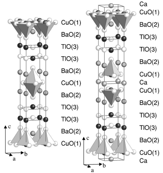
FIG. 4. Crystal structure of \text{Tl}_2\text{Ba}_2\text{CuO}_6 (left) and \text{Tl}_2\text{Ba}_2\text{CaCu}_2\text{O}_8 (right).
