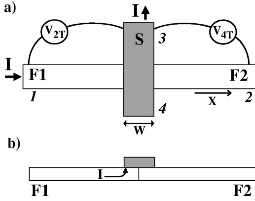
FIG. 1. (a) Top view of a cross type F/S geometry. S is the superconducting strip on top of two ferromagnetic strips F1 and F2 . The magnetization of F2 can be parallel or antiparallel to the magnetization of F1 . The x axis is taken along the ferromagnetic strips, where from x=0 to x=W the superconducting strip covers the ferromagnetic strips. (b) Side view.
