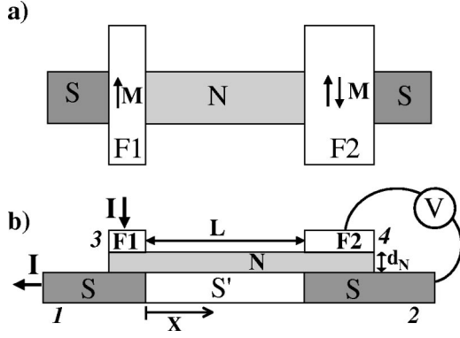
FIG. 3. (a) Top view of an F/N/S geometry. N is a normal metal strip coupling to the two superconducting strips S . In the region S' a superconductor may be present (see text). On top of the normal metal two ferromagnetic strips F1 and F2 are placed. (b) Side view, terminals 3 and 1 are used for current injection and extraction, whereas terminals 2 and 4 measure the voltage. M refers to the magnetization of the ferromagnetic electrodes F1 and F2 . L is the distance between the two ferromagnetic electrodes and d_N is the thickness of the normal metal.
