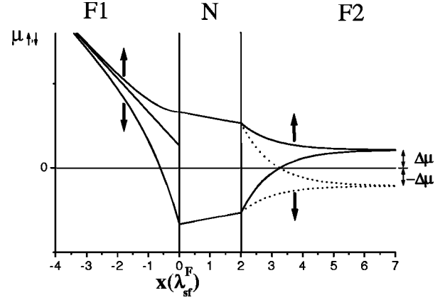
FIG. 4. Electrochemical potential versus distance. The coordinate x=0 defines the position of the ferromagnetic electrode F1 . The coordinate x=L=2\lambda_{sf}^F defines the position of the ferromagnetic electrode F2 . The solid curves for x>L yield the chemical potentials for the two spins when the ferromagnetic electrode F2 is magnetized parallel to the magnetization of F1 . The dotted curves yield the chemical potentials for antiparallel magnetization.
