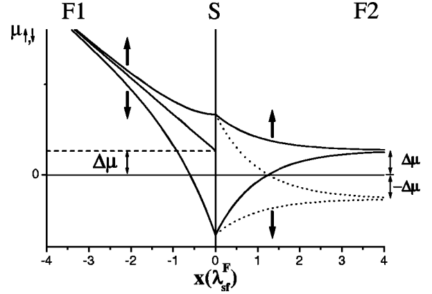
FIG. 2. Electrochemical potential in the ferromagnetic strip of Fig. 1 as a function of distance along the x axis in units of the spin-flip length \lambda_{sf}^F . The potential of the superconductor at x=0 is set to zero. The solid curves at x>0 yield the chemical potentials for the two spin directions when the ferromagnetic electrode F2 is magnetized parallel to the magnetization of F1 . The dotted curves yield the electrochemical potentials for antiparallel magnetization.
