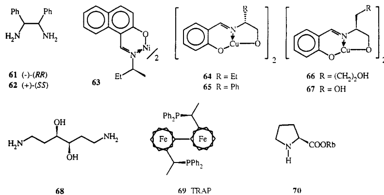
Figure 17. Chiral ligands and complexes used as catalysts in enantioselective Michael additions.
