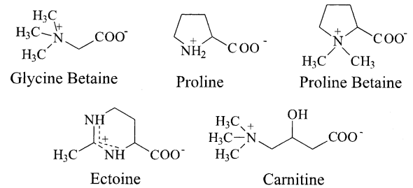
Fig. 1. Structures of selected compatible solutes.
