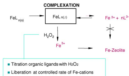
Fig. 5. Complexation of Fe with carboxylic ligands hinders the exchange process. Not all the Fe is exchanged. By using H 2 O 2 , the ligands can be oxidized and Fe is released at a controlled rate.
