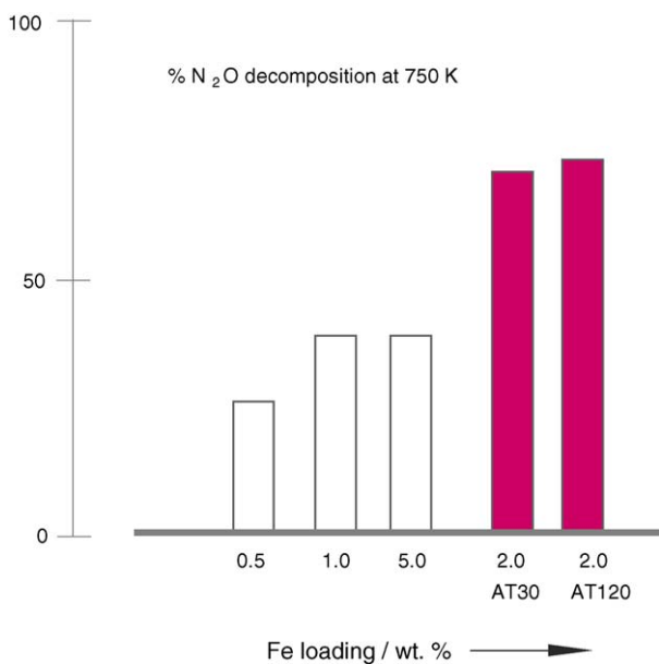
Fig. 4. Effect of the targeted iron loading on N 2 O decomposition activity for the ZSM5 system. Hollow bars correspond to the untreated Fe-ZSM5 catalysts, while the filled ones are the Fe-AT catalysts. Reaction conditions: 4.5 mbar N 2 O, He balance at 3 bar-a total pressure and W/F 0 (N 2 O) = 900 kg s mol -1 .
