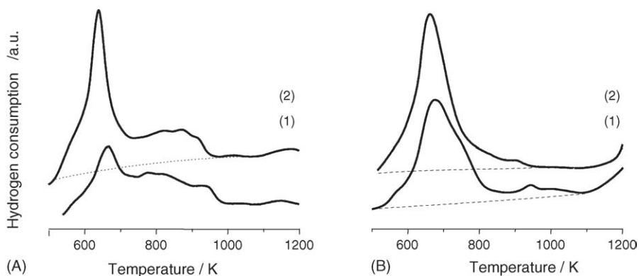
Fig. 3. H 2 -TPR profiles of: (A) the untreated Fe-ZSM5 catalysts, (1) 0.5 wt.% Fe and (2) 5.0 wt.% Fe, both targeted and (B) profiles for the alkaline modified catalysts, (1) Fe-AT-30 and (2) Fe-AT-120. Conditions: 5% H 2 /Ar; ramp. 10 K/min.
