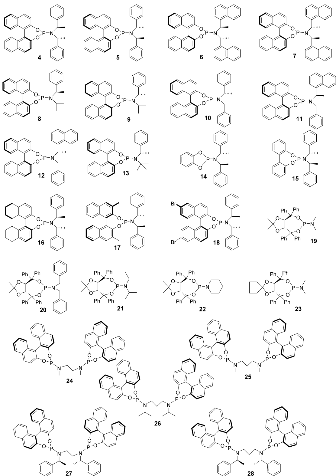
Scheme 4. Chiral phosphoramidite ligands applied in Cu-catalyzed allylic alkylation.
