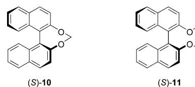
Figure 3. Model compounds ( S )- 10 and ( S )- 11 .
