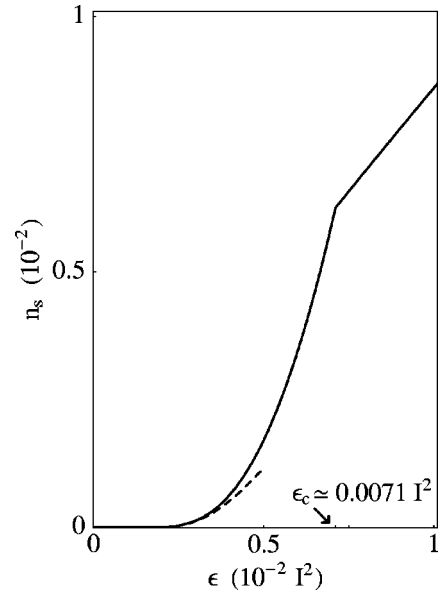
FIG. 4. Density of spin flips within the chains of the anisotropic RFIM as a function of the random magnetic-field strength at T = T_0 , i.e., in the ground state. The interchain interaction was chosen such that \tilde{I}_\perp/I = 0.02 . The dashed line shows the analytical result Eq. (67) for \epsilon \ll \epsilon_c \approx 0.0071 I^2 .
