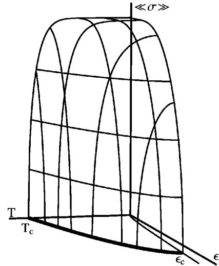
FIG. 2. The order parameter \langle\langle\sigma\rangle\rangle of the anisotropic RFIM as a function of the random magnetic-field strength \epsilon and temperature T [for T > T_0(\epsilon) ]. The plot was obtained by solving the self-consistency condition Eq. (11) with the analytical solution Eq. (40) for the free energy. The interchain interaction was chosen such that \tilde{I}_\perp/I = 0.02 , in which case T_c \approx 0.295I (at \epsilon = 0 ) and \epsilon_c = 0.0071I^2 . At (T, \epsilon) = (0, 0) , the order parameter reaches its maximum: \langle\langle\sigma\rangle\rangle = 1 . The thick curve in the \langle\langle\sigma\rangle\rangle = 0 plane separates the (\epsilon, T) regions with and without LRO.
