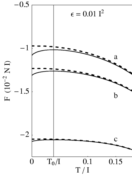
FIG. 1. The average free energy of the anisotropic RFIM as a function of temperature for three values of the mean field: B = 0.005I , 0.01I , and 0.02I (curves a, b, and c, respectively). Solid curves represent the analytical result Eq. (40) for the continuum approximation to the RFIM; dashed curves are obtained from numerical simulations of the RFIM. In all cases, the random field strength was taken \epsilon = 0.01I^2 . The thin line at T = T_0 gives the position of the maxima of the analytical solution.
