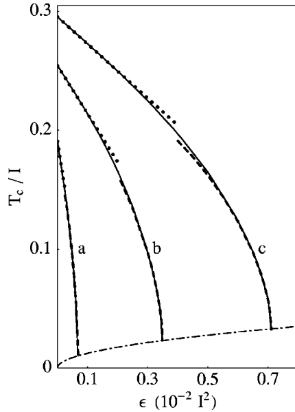
FIG. 3. The critical temperature T_c(\epsilon) of the anisotropic RFIM as a function of the random magnetic-field strength for \tilde{I}_\perp/I = 0.002, 0.01, and 0.02 (curves a, b, and c, respectively). Solid curves derive from solving Eq. (11) with the exact free energy Eq. (40). The dashed curves are obtained by solving Eq. (61), while the dots represent the small- \epsilon behavior Eq. (49). The dash-dotted curve shows the temperature T_0(\epsilon) , below which the continuum approximation breaks down and which corresponds approximately to T = 0 in the discrete RFIM.
