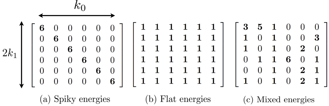
Figure 1: Three hypothetical examples of matrices with (r, j) -th entry given by |\widehat{Z}_j^r|^2 , i.e., each row corresponds to a single sequence Z^r , but only at the entries corresponding to the k_0 blocks in X .
