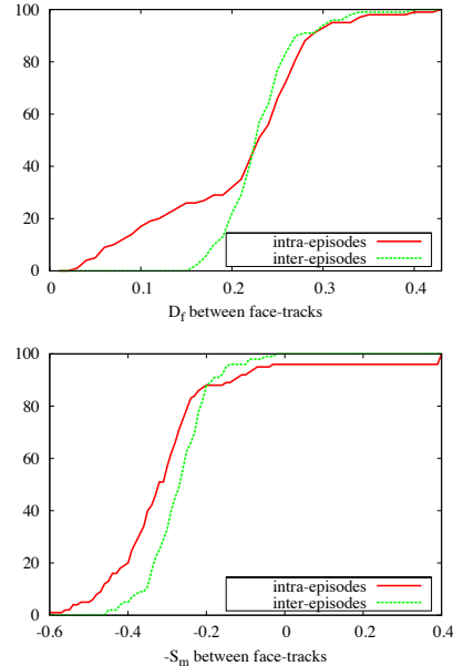
Figure 5: Cumulative percentage of tracks pairs from the character Joyce whose pairwise (dis)similarity measures are below a given threshold for the D_f (top) and (-S_m) (bottom) measures when considering track pairs within an episode or between an episode.
