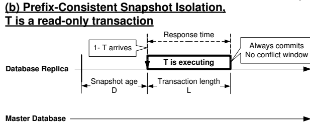
Figure 1. Transaction execution in replicated database using PCSI with master database & centralized certification.
