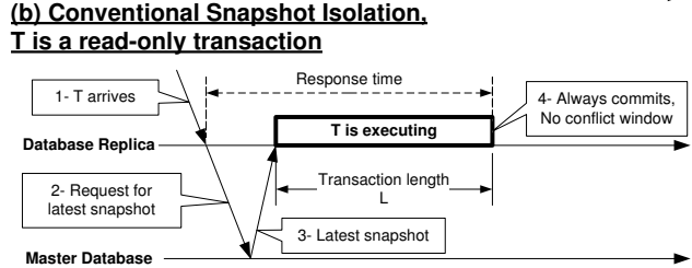
Figure 2. Transaction execution in replicated database using CSI with master database & centralized certification.
