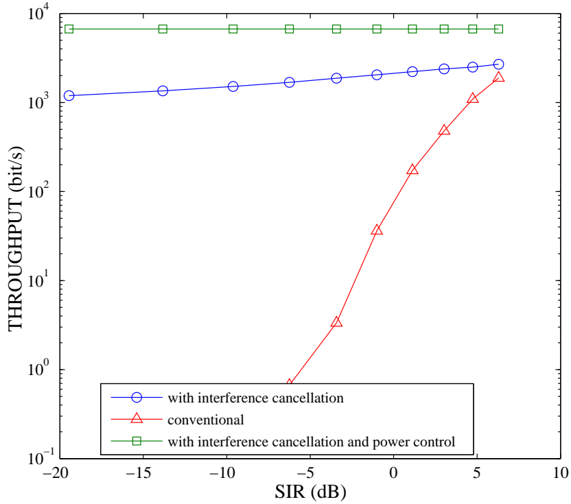
Fig. 3.5 FUE's throughput from power control by the femtocell.
