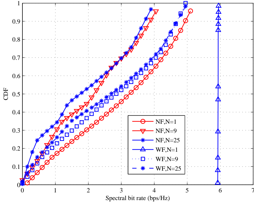
Fig. 4.7 Spectral bit rate at sensor Node and FBSs with |\Omega_M| .
