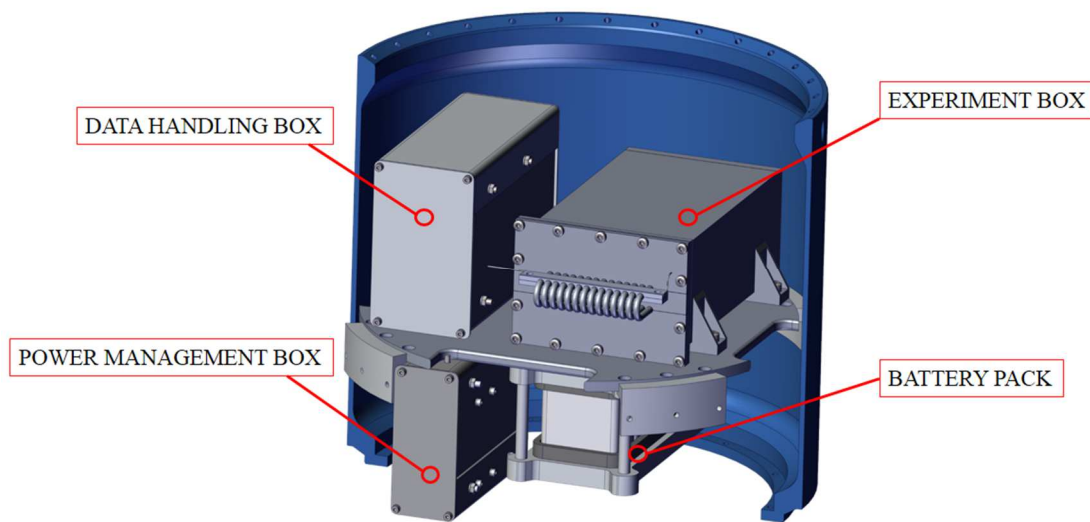
Figure 2 Experiment Assembly.
