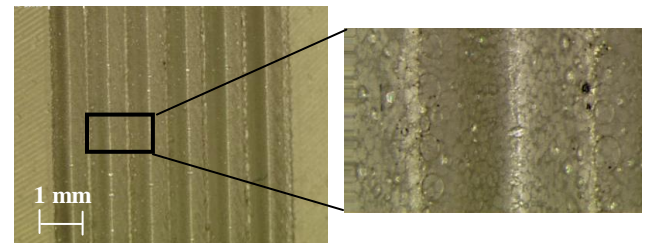
Fig. 10. Multiple scans on PMMA with f=200 mm, W=27.1 W, v=110 mm/s and p_s=0.8 mm.
