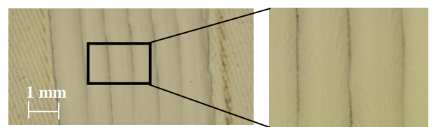
Fig. 11. Multiple scans on Zirconia with f=180 mm, W=27.1 W, v=25 mm/s and p_s=0.8 mm.
