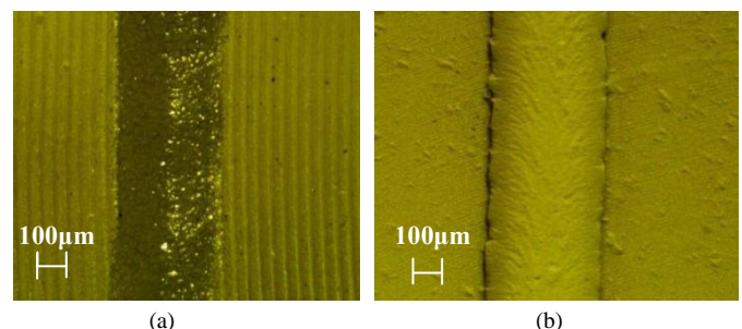
Fig. 5. Single scan captured with optical microscope. Groove on: (a) PMMA ( f=180 mm; W= 22.5 W v=20 mm/s); (b) Zirconia ( f=180 mm; W= 28.3 W, v=20 mm/s).
