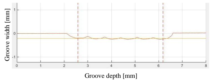
Fig. 10. Multiple scans on PMMA with f=200 mm, W=27.1 W, v=110 mm/s and p_s=0.8 mm.
