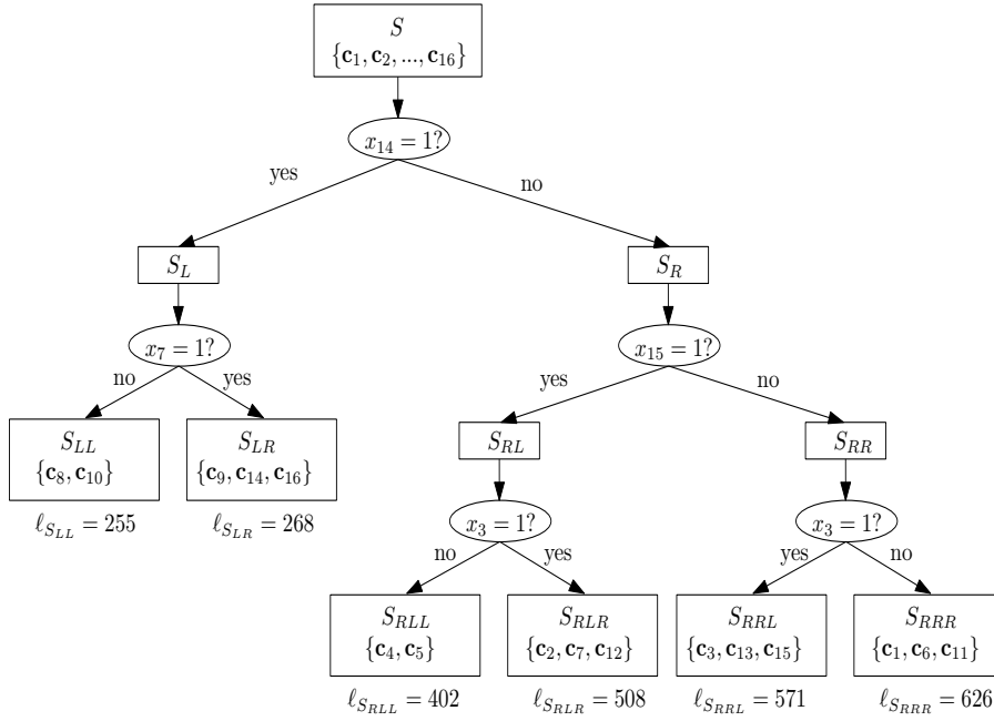
Figure 2 A sample prediction model of x264 learned by CART from the example of Table 1
