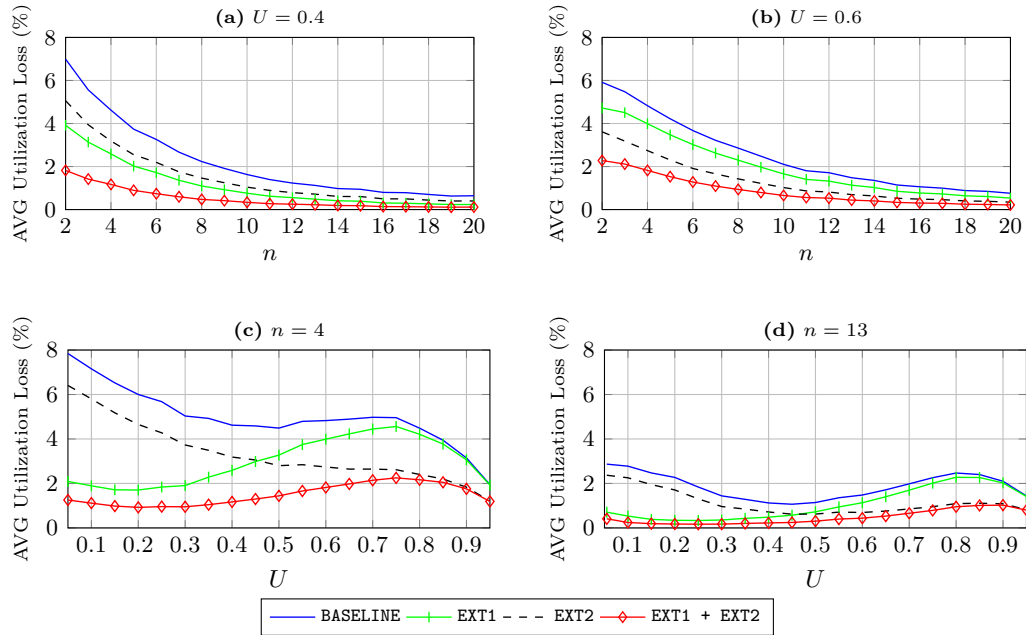
■ Figure 3 Average utilization loss introduced by the approximate algorithms for C=D splitting (presented in Section 3) as a function of the number of reservations n (insets (a) and (b)) and the utilization U (insets (c) and (d)). The results are related to four representative configurations identified by the fixed parameter reported in the caption above the graphs.
