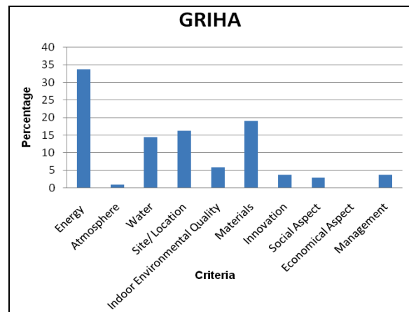
Figure 7. Weightings of green building criteria in GRIHA Source: Own illustration
