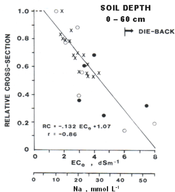
Fig. 1 Trunk cross-section as affected by salinity or Na concentrations in the soil saturation extract (Miyamoto, 1986).
