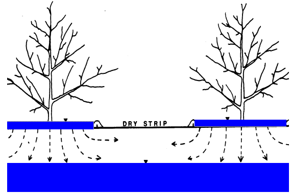
Fig. 4. Strip leaching of salted orchard with a high water table
