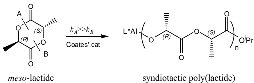
Figure 2-5. Syndiotactic poly(lactide) from the ring-opening polymerization of meso -lactide using Coates' catalyst.
