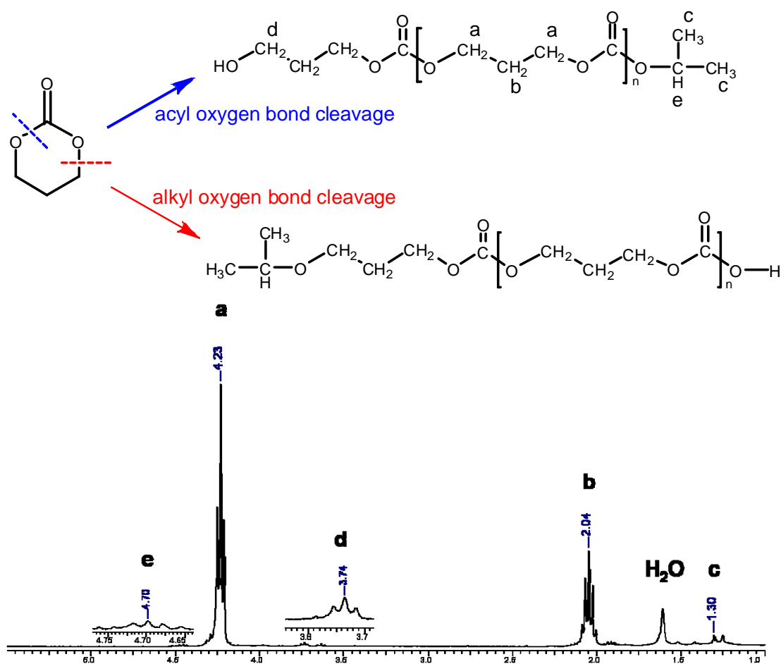
Figure 2-20. ^1\text{H} NMR spectrum of poly(TMC) terminated by 2-propanol.
