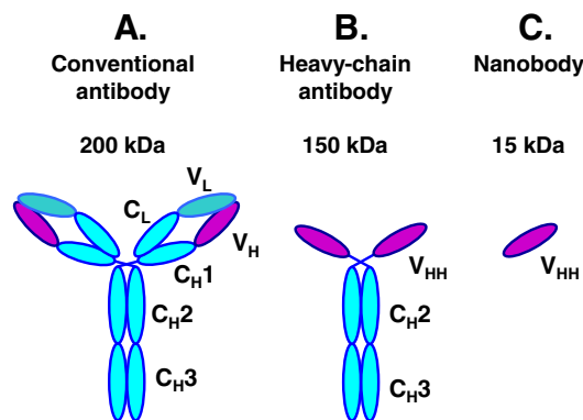
Fig. 2. Scheme of a conventional IgG antibody. (A), a camelid heavy-chain IgG antibody (B) and the variable domain of heavy chain antibodies, VHH, also known as a nanobody (C). Conventional antibodies have two identical heavy chains, formed by V_H , C_{H1} , C_{H2} and C_{H3} domains and two identical light chains, V_L and C_L domains. Heavy-chain antibodies contain a single V_{HH} and two constant domains ( C_{H2} and C_{H3} ). A Nanobody is the V_{HH} domain of heavy-chain antibodies obtained by recombinant gene technology. C_{H1} – C_{H3} : constant domains of heavy chain. C_L : constant domain of light chain. V_H : variable domain of heavy chain. V_L : variable domain of light chain.
