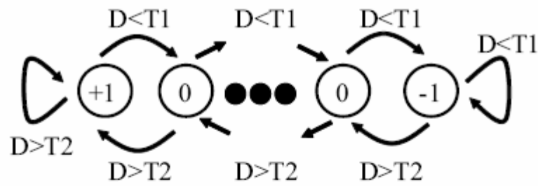
(a) N-Bit Symmetric State Machine
