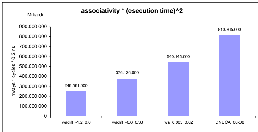
Figura 4.23 - Statistiche associativity * (esection\ time)^2 relative a bzip2
