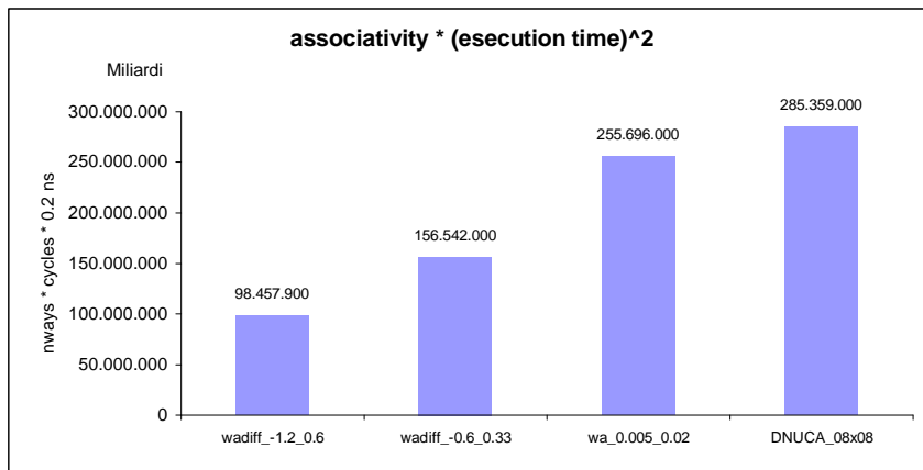
Figura 4.33 - Statistiche associativity * (esection time)^2 relative ad equake
