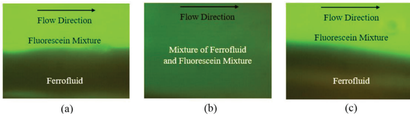
Figure 5: Single-phase flow visualization – enhanced magnetic mixing results. (a) No magnetic field; (b) Magnet position 1; (c) Magnet position 2.
