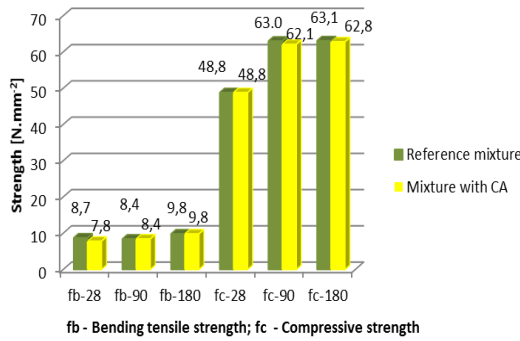
Fig. 2 Determination of strength of specimens stored in water
