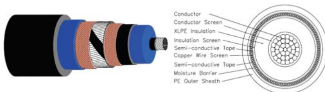
Fig. 3 Single core submarine power cable cross section [3]
