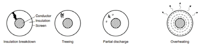
Fig. 5 Internal threats [5]
