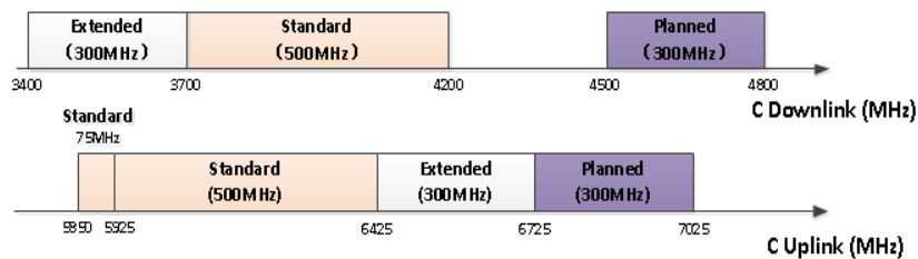
Fig. 2 C band allocation
