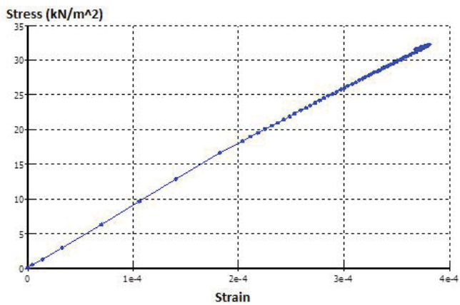
Fig. 6 Stress – Strain Curve at Midpoint of Footing
