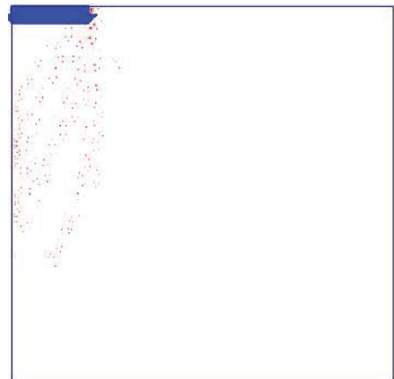
Fig. 7 (b) Total incremental strain contours
