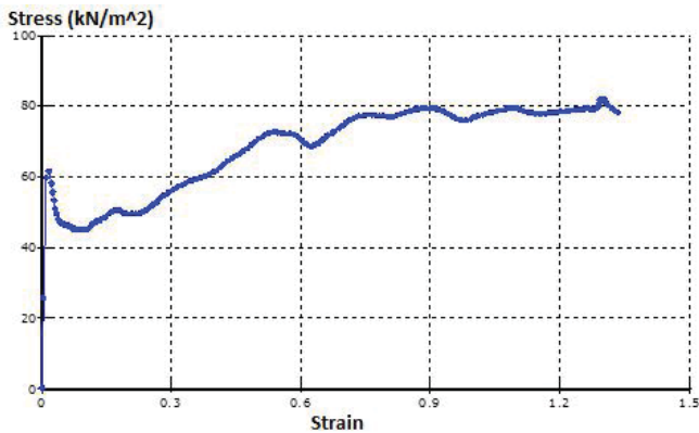
Fig. 5 Stress – Strain Curve at Edge of Footing
