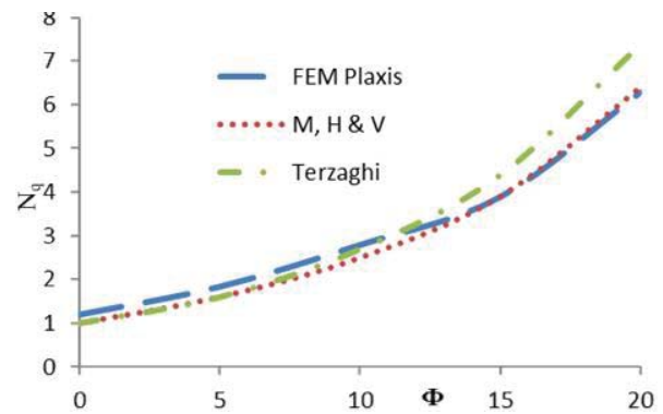
Fig. 11 Analytical and Numerical Values of N_q
