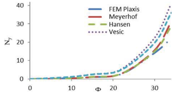
Fig. 10 Analytical and Numerical Values of N_\gamma
