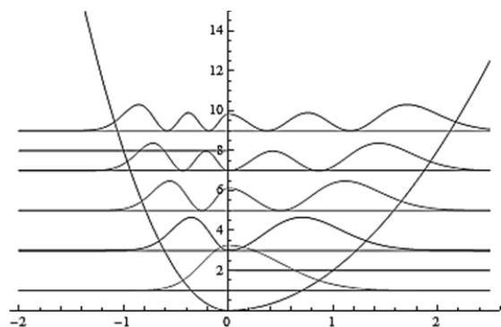
Fig. 3 Potential (32), the probability density |\psi_n(x)|^2 given in (33), the energy spectra E_n = \beta(2n + 1) , n = 0, 1, 2, 3, 4 and the mass distribution m(x) given in (28). m_1 = 8, m_2 = 2, x_0 = 0, \beta = 1 and \hbar = m_0 = 1
