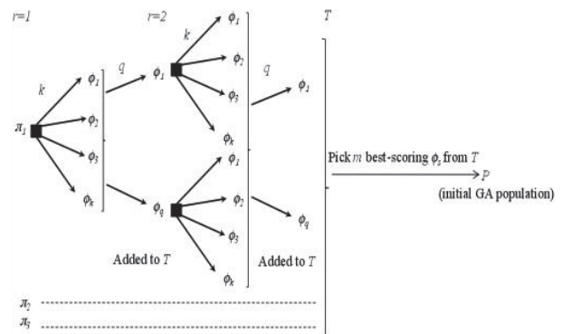
Fig. 2 Initialization Phase
