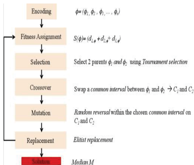
Fig. 3 Genetic Algorithm
