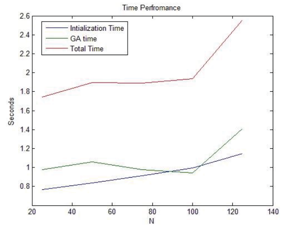
Fig. 11 The time performance of the median score found through five experiments of i=6 with five different values of n : 25, 50, 75, 100 and 125, where k = 14 , q = 7 , the size of priority queue T is 30
