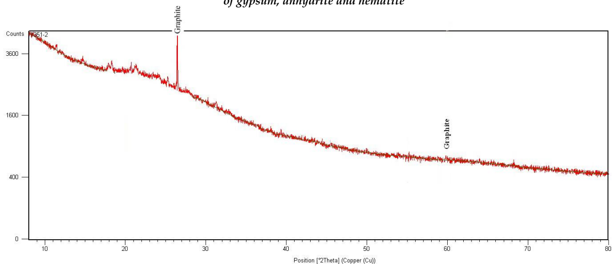
Figure 7. X-ray diffraction spectrum of previous conservation material shows the presence of graphite in the black resinous material.
