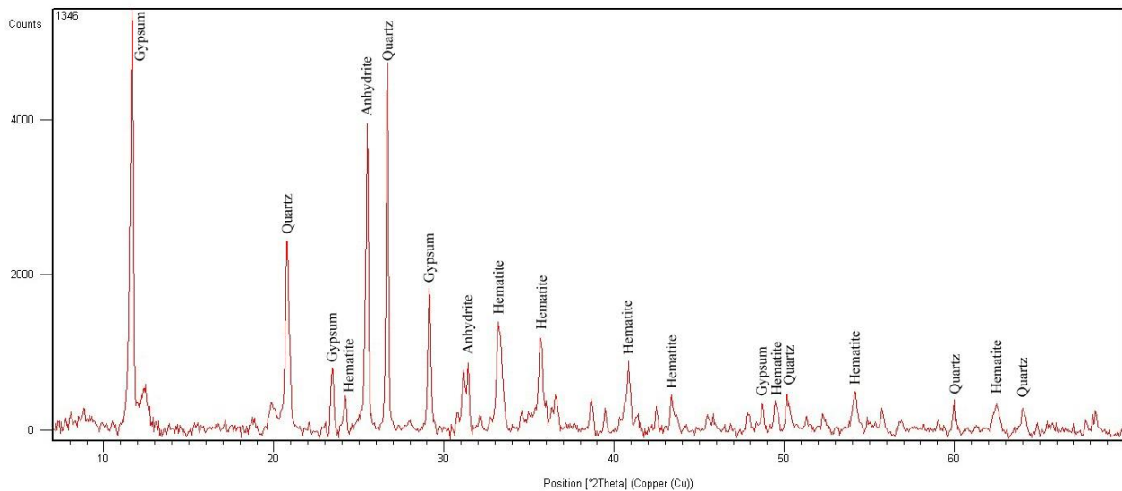
Figure 6. X-ray diffraction spectrum for previous conservation material showing the filling material is a mixture of gypsum, anhydrite and hematite
