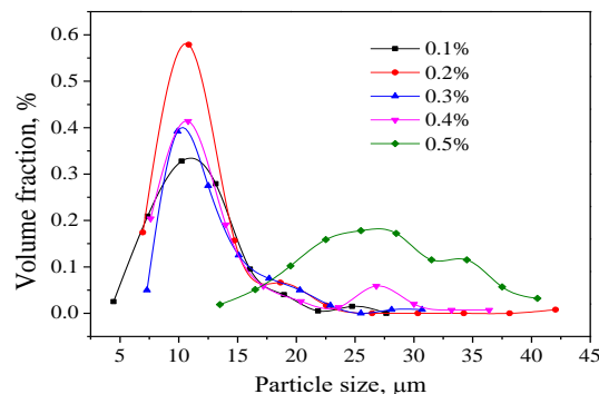
Fig. 3. Effect of PVA concentration on the distribution of the microcapsules size
