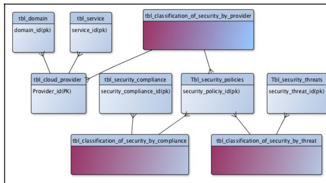
Figure 2: Database architecture for the application
