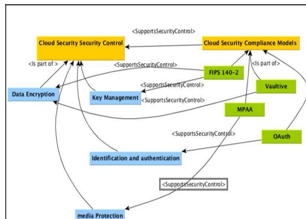
Figure 1: Ontology describing relationship between Security Controls and security Compliance classes.
