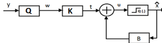
Figure 1 DFE architecture.
