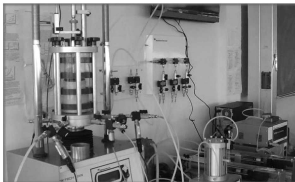
Fig. 4. Experiment device
