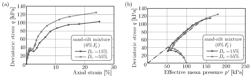
Fig. 6. (a) Test results of deviatoric stress versus axial strain ( q, \varepsilon_a ), F_c = 0\% , (b) stress paths ( q, p' ) for undrained loading tests, F_c = 0\%
