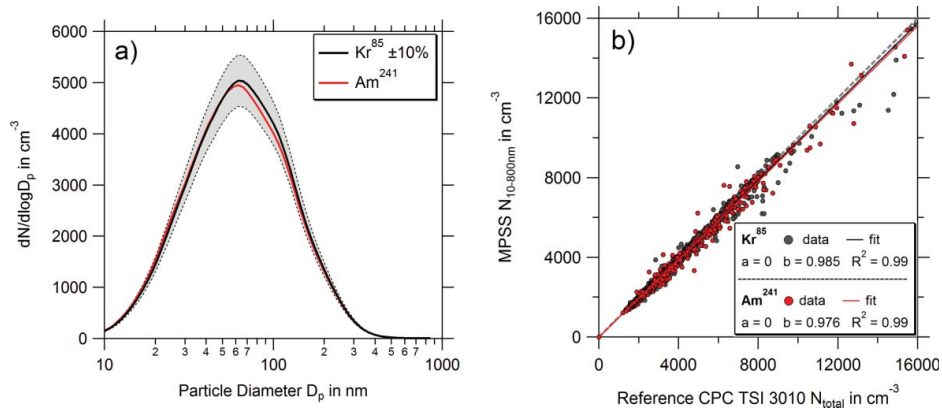
Figure 12. Intercomparison of a \text{Kr}^{85} (370 MBq) and a \text{Am}^{241} (74 MBq) bipolar diffusion charger. The PNSD of the candidate is within the \pm 10\% target uncertainty compared to the reference MPSS (a). The integrated PNC of the candidate and reference MPSS are within \pm 10\% uncertainty range against the reference CPC (b). Time resolution of the data is 10 min.
