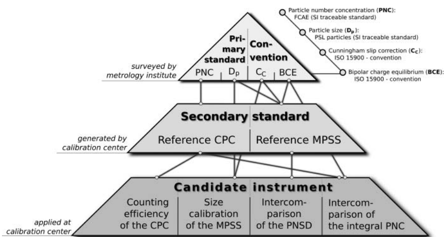
Figure 1. Traceability of MPSS measurements to a set of certified standards and conventions. To facilitate the time-efficient calibration of candidate instruments, intermediate standards (so-called “reference instruments”) are used at the calibration center.
