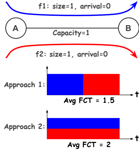
Fig. 5. It may not be possible to optimize all performance metrics together (mismatch between fairness and mean FCT)
