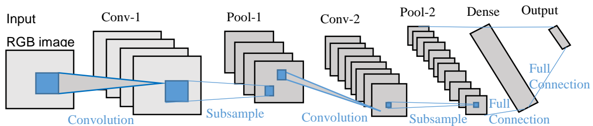
Figure 2. The LeNet architecture
