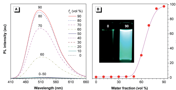
Fig. 2 (A) PL spectra of TPE–NPB in THF and water mixtures with different water fractions ( f_w ). (B) Plot of the relative PL intensity ( I/I_0 ) versus the composition of THF–water mixture of TPE–NPB. I_0 = emission intensity in pure THF solution. Concentration: 10 \mu M; excitation wavelength: 340 nm. Inset in (B) are the fluorescent photographs at f_w = 0 and 90% taken under 365 nm UV irradiation from a handheld UV lamp.
