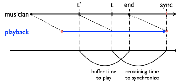
Figure 5: The diagram represents the different values to be considered for the speed calculation. At the current time t , the dates end (the canon end) and sync (the final synchronization point) are estimated according to the tempo value. The t' value corresponds to the time at which the live musician played the current position of the buffer.
