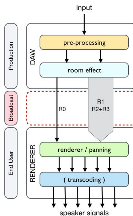
Figure 13: General signal-based metadata scheme for the channel-based and scene-based reverberation on object-based audio.
