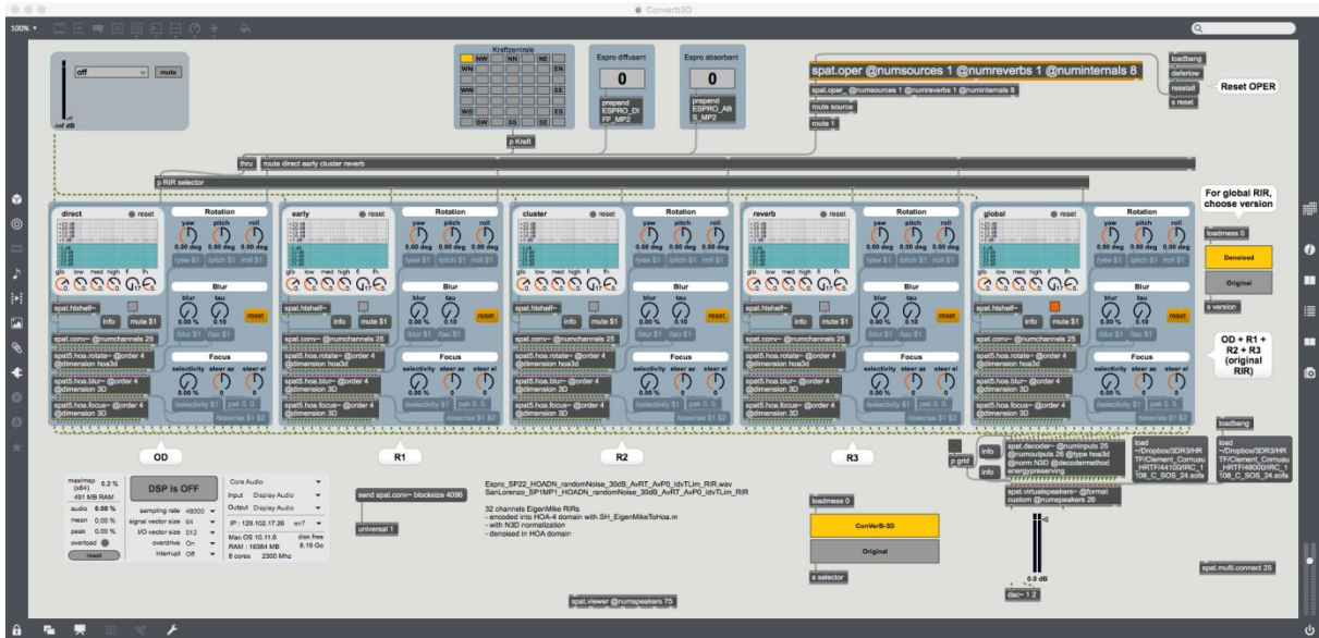
Figure 17: IRCAM Spat~ implementation of a convolution-based DRIR reverberation processor with perceptual control.
