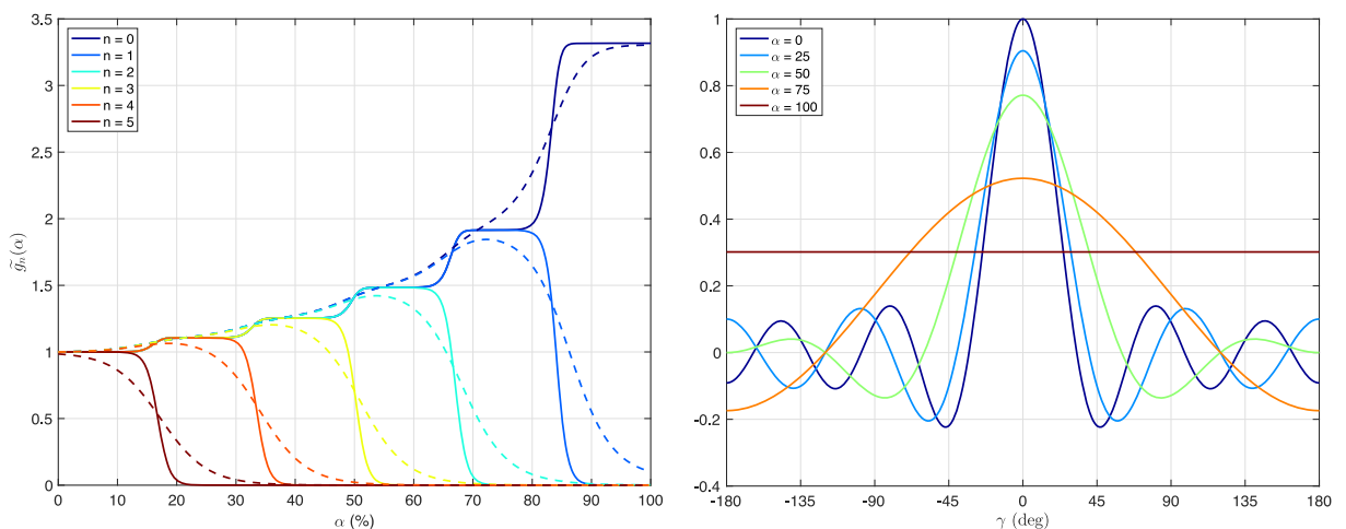
Figure 14: Energy preserving weighting functions (left) and order dependent panning function (right) as a function of the spatial blur factor \alpha (in percent) for spherical harmonic orders up to N=5 .
