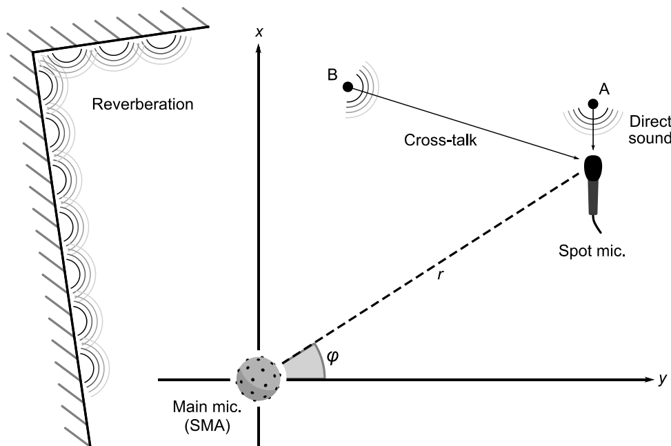
Figure 6: Problem setup: estimating the location of source A by analysing the signals recorded by the “Main” and “Spot” microphones (please refer to text for more details).
