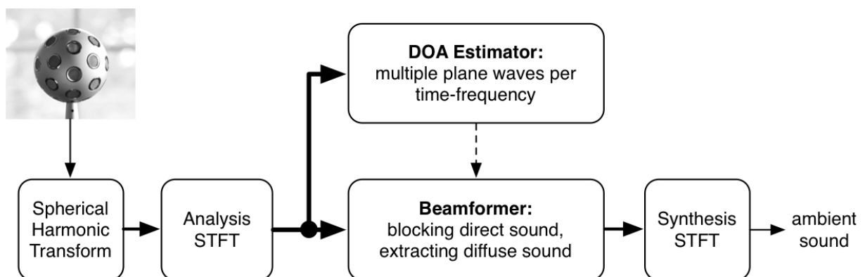
Figure 12: Block diagram of the ambient sound capturing algorithm
