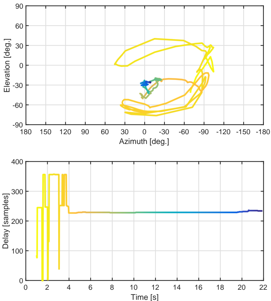
Figure 9: Trace of the source localisation algorithm's output when run on recorded signals. The colour of the line indicates at which point in the signals the position and delay were estimated.
