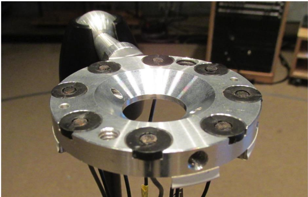
Figure 1: Example of a cylindrical microphone array
