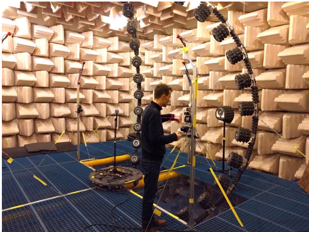
Figure 4: Setting up the acoustic characterisation of an SMA in the HRTF measurement facility.
