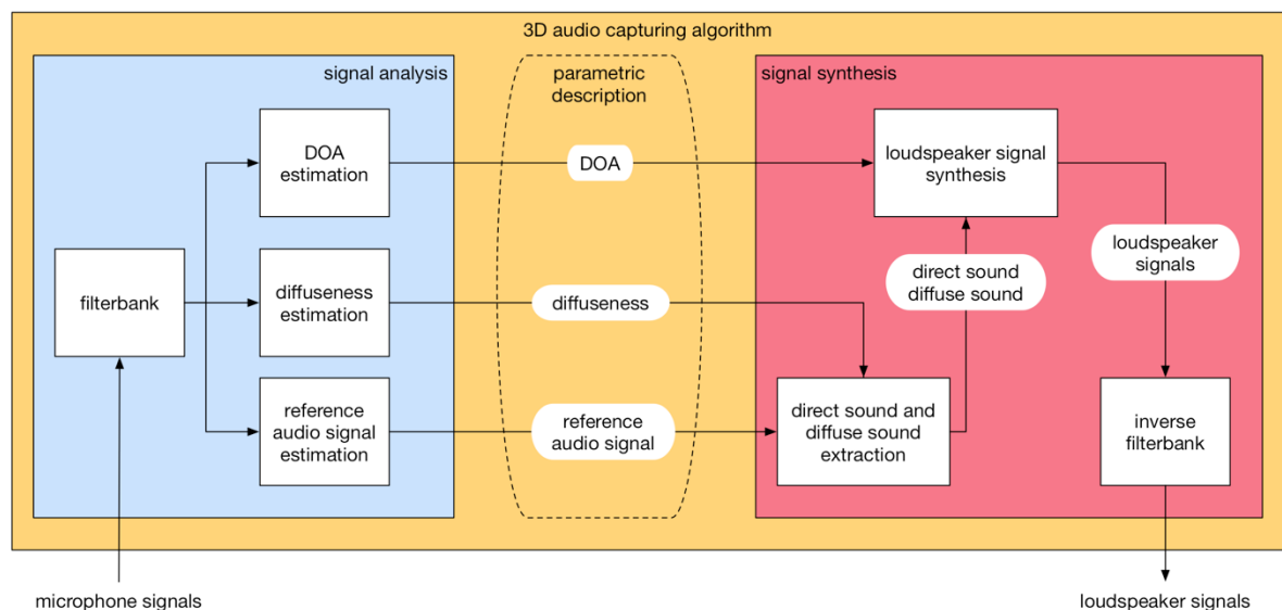
Figure 2: Block diagram of the 3D audio capturing algorithm
