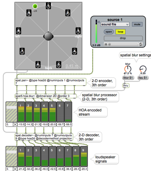
Figure 15: Implementation of the spatial blur function in the IRCAM Spat~ real-time processing environment.
