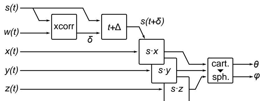
Figure 7: Flow diagram of the MainSpot algorithm.
