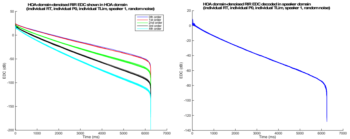
Figure 16: DRIR of the Chiesa San Lorenzo after de-noising in the HOA domain. Energy decay curve of the denoised DRIR in the HOA domain (left) and in the spatial domain (right).
