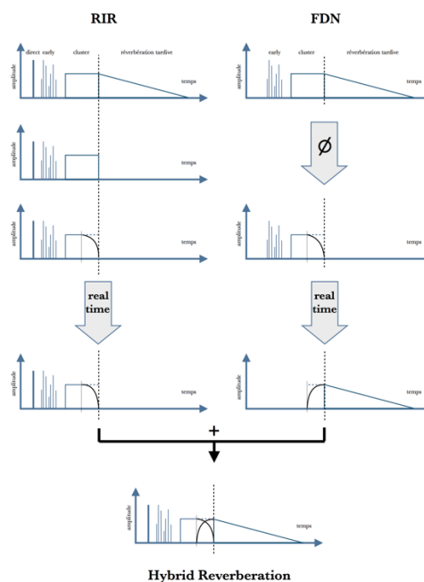
Figure 18: Hybrid reverberation processing with crossfade.
