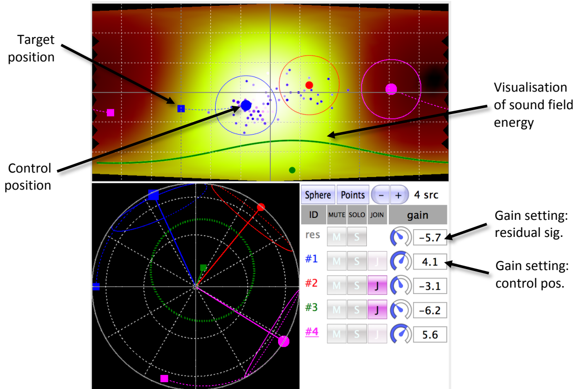
Figure 11: User interface for b<>com's Sound Field Editor VST plugin.
