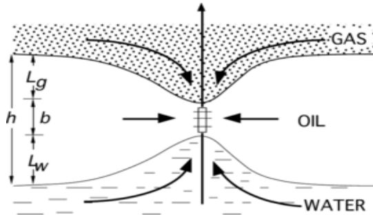
Fig. 2. Gas and water coning schematic in producing well [16]
