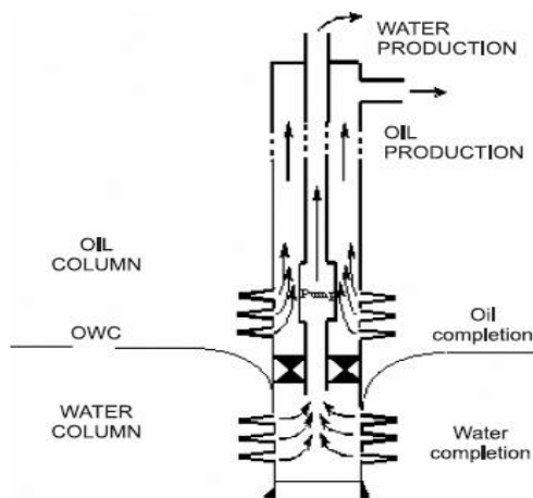
Fig. 5. Downhole water sink schematic [91]
