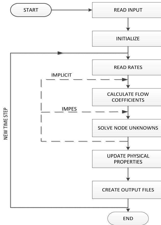
Fig. 1A. Typical numerical simulation flowchart [103]
