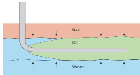
Fig. 3. Horizontal well schematic [82]
