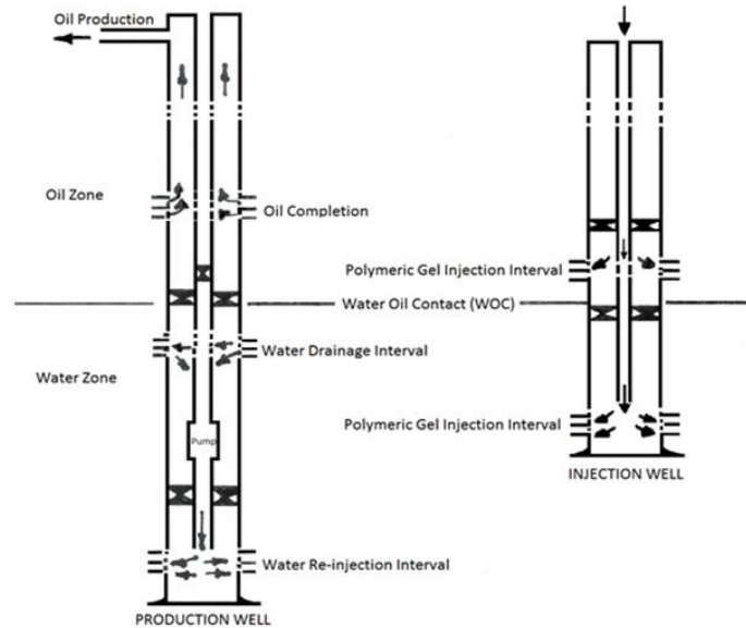
Fig. 8. Well completions of the proposed integrated approach
