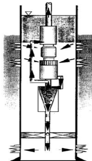
Fig. 4. Downhole oil-water separation schematic [89]
