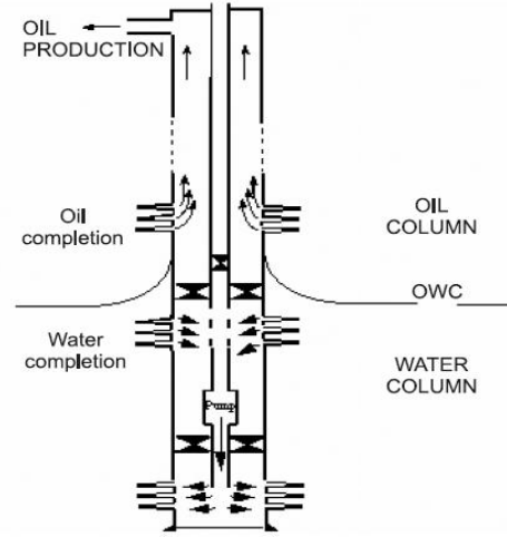
Fig. 6. Downhole water loop schematic [91]
