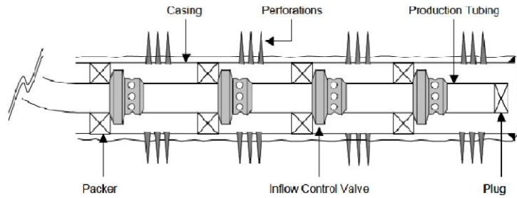
Fig. 7. Intelligent well completion schematic [98]
