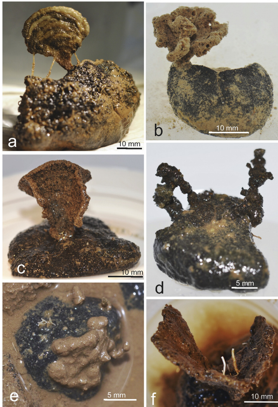
Fig. 2. Selected xenophyophores associated with nodules. (a) Psammmina limbata ; Cruise AB01, UK-1 area, Stratum A, Site F. (b) Galatheaammia sp. 8; Cruise AB02, OMS area, Site S02. (c) Galatheaammia sp. 5; Cruise AB02, UK-1 area, Stratum B, Site U12. (d) Aschemonella sp. nov. 1; Cruise AB02, UK-1 area, Stratum B, Site U01. (e) Xenophyophore sp. 3; Cruise AB02, UK-1 area, Stratum B, Site U13. (f) Galatheaammia sp. 5 with attached polychaete (serpulid) tubes; Cruise AB01, UK-1 area Stratum A, Site I.
