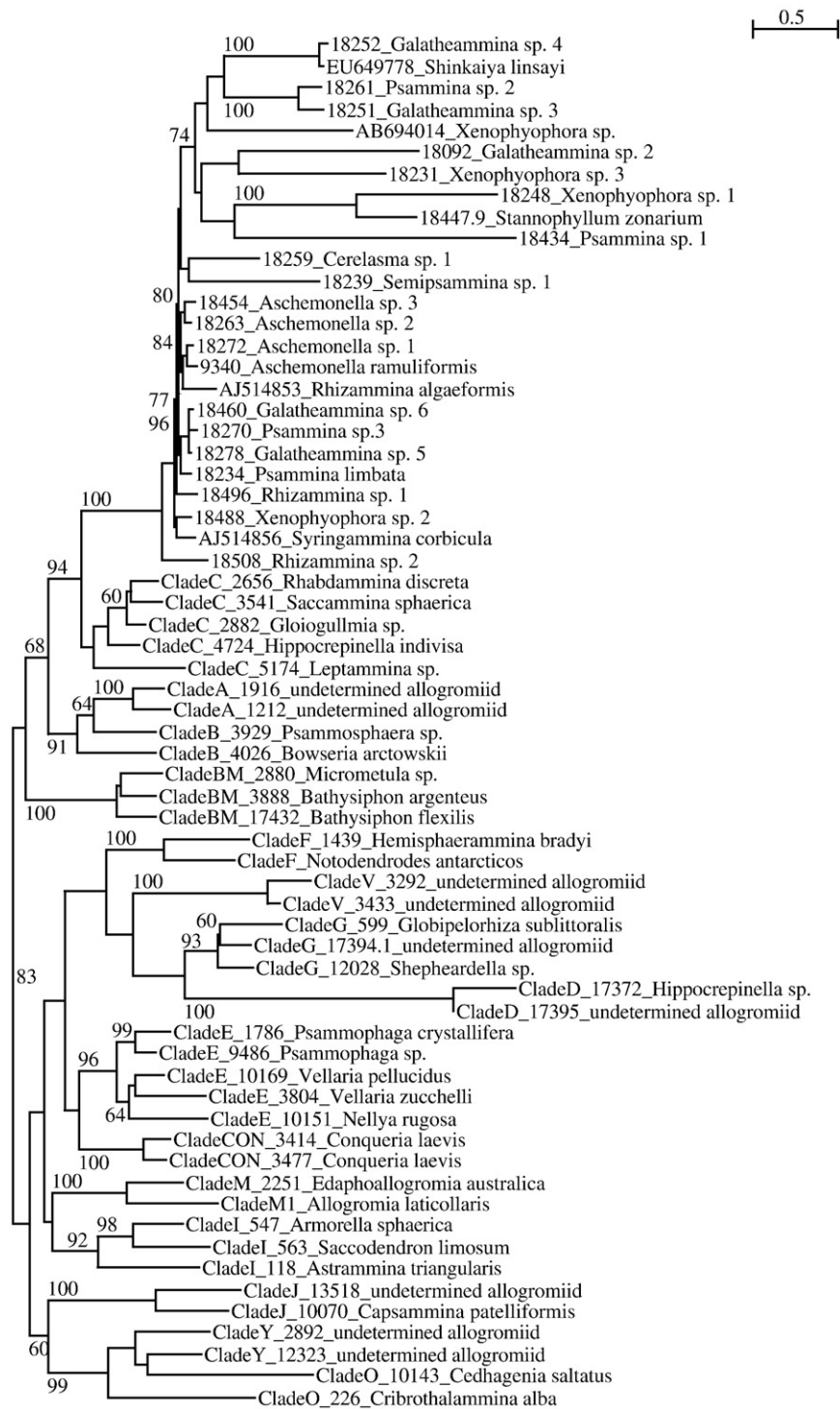
Fig. 5. PhyML phylogenetic tree showing evolutionary relationships of 25 xenophyophore species (20 from ABYSSLINE material) and 39 monothalamid sequences belonging to clades C, A, B, BM, F, V, G, D, E, CON, M, M1, I, J, Y and O. The tree is unrooted. Numbers at nodes indicate bootstrap values.
