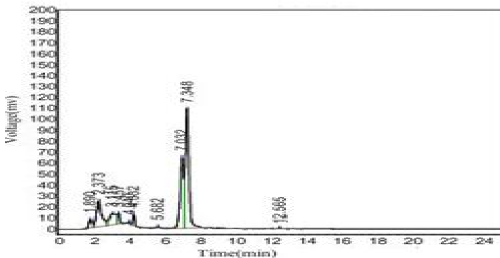
S -HPLC chromatogram of TT1-1Fig
