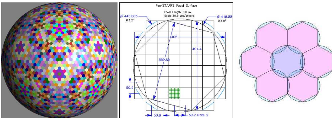
Figure 4: Left: Outside view of the celestial sky tessellated into 6252 fields. Of these fields, 5464 have boresight centers \geq -30 degrees Declination. Center, the 3 degree field of view of PS1 with an inscribed hexagon of 5.84 square degrees. Right, the twenty percent overlap from a single tessellation due to the circular field of view.
