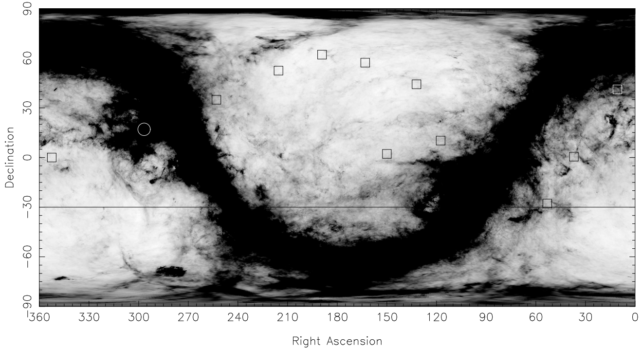
Figure 3: Celestial sphere in Mercator projection showing extinction map from WMAP. The proposed Medium Deep Fields are marked as black boxes, the white circle is one of the stellar transit fields, and the white square is M31. The black line at -30 degrees Declination shows the southern limit of the PS1 3\pi Steradian Survey pointing centers.
